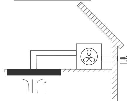
Internal in-roof motor with round ducting
