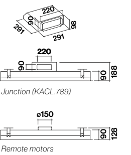
Remote motors
