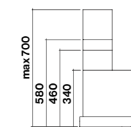
Side view with optional chimney
