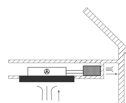
Slim motor with Carbon.Zeo vertical filter unit
