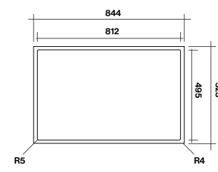
Flush installation Cutout size
