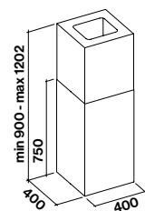
Island version
