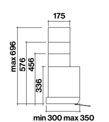
Side view with optional chimney
