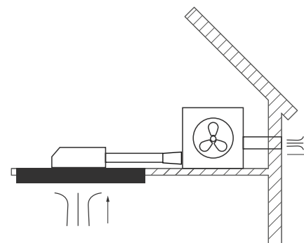
Indoor in-roof motor with flat ducting
