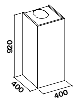
Wall version
