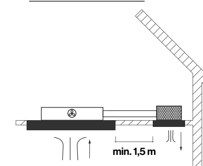
Slim motor with Carbon.Zeo filter unit.
