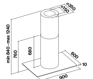
Island version with glass (optional)
