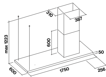
Right version
