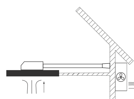
External extractor fan with flat ducting
